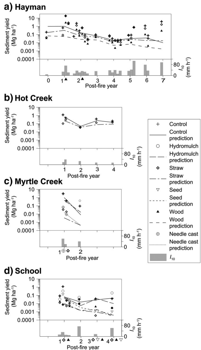
Fig. 6. The observed event and predicted annual sediment yields vs. number of post-fire years and maximum 10-min rainfall intensity ( I_{10} ) for each fire: a) Hayman; b) Hot Creek; c) Myrtle Creek; and d) School. Only the post-fire years with complete rainfall data were modeled and are shown. The bars represent the I_{10} associated with the mean observed sediment yields for each event. Predicted annual sediment yields are shown with lines (style varies by treatment). Treatment symbols located next to the post-fire year labels on the X-axis indicate significant differences ( \alpha=0.05 ) in modeled mean annual sediment yields between the treatment indicated by the symbol and the controls in that post-fire year. Wheat straw mulch is referred to as “Straw” and wood strand mulch is referred to as “Wood” in the legend.
