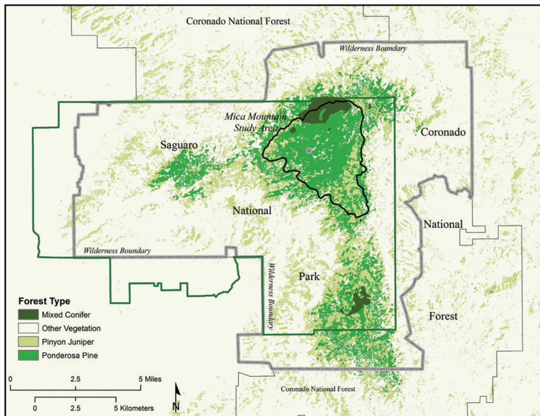
Figure 6 —Maps of vegetation communities in (a) the Gila and Aldo Leopold Wilderness Complex and surrounding lands, and (b) Saguaro National Park. Vegetation categories are derived from Landfire Data ( www.landfire.gov ; last accessed 1/21/14).
