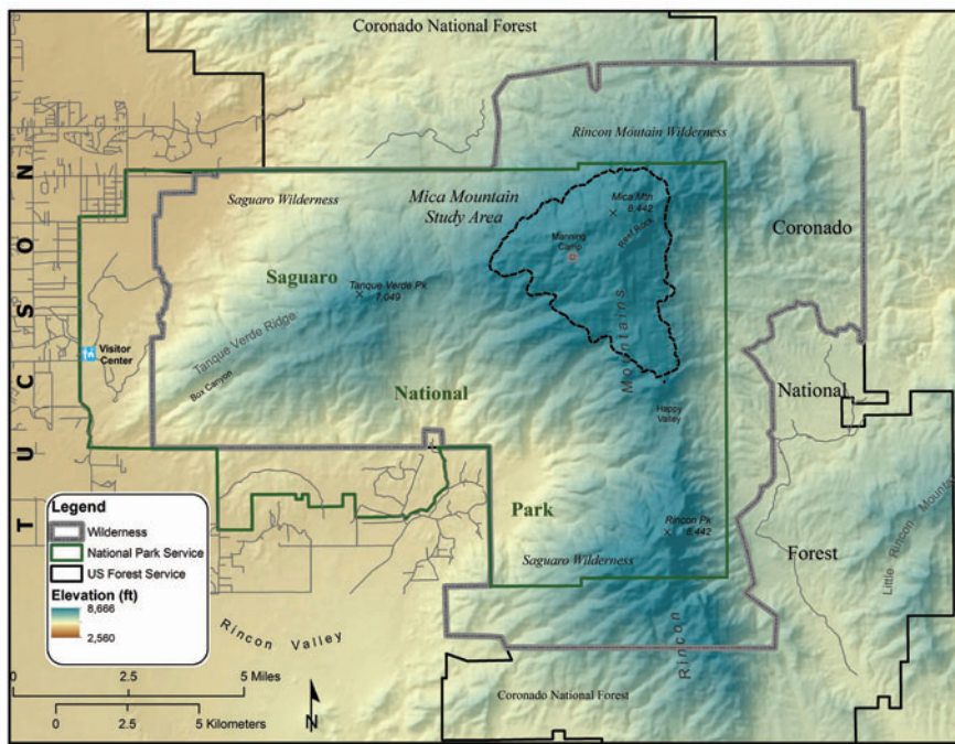
Figure 3 —Detailed map of the Saguario Wilderness Area in Saguario National Park and the adjacent Rincon Mountain Wilderness Area in the Coronado National Forest. The outlined Mica Mountain Study Area represents a 6,870 acre area on Mica Mountain where the prescribed fire and managed wildfire program has been focused. It is also where most fire history studies have been conducted.
