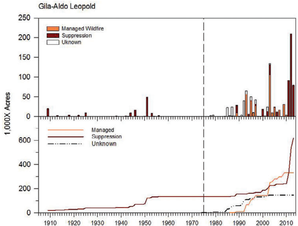
Figure 16 —Area burned per year in the Gila and Aldo Leopold Wilderness Complex since 1909. The top panel shows annual area burned, and the bottom panel shows cumulative area burned in managed wildfires, suppression fires, and fires of “unknown” status (fires in which there was no information available in the database). Vertical dashed line indicates first year of managed wildfire in 1975. Prescribed fires have not occurred within these wilderness areas. The graph includes only fires greater than 100 acres.
